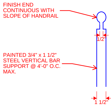
END SUPPORT ELEVATION
